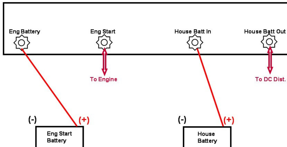
T.A.B.S 1 Eng. 2 Batt. Model Wiring
