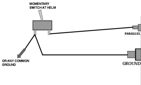
PARALLEL SWITCH WIRE DIAGRAM
